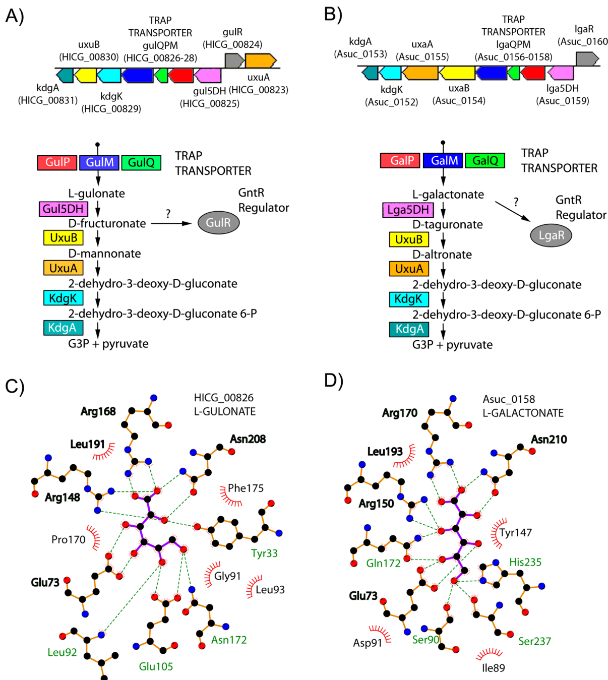
Figure 6. Functional implications from L-galactonate/L-gulonate TRAP SBPs. (A) Genome context of HICG_00826, a TRAP SBP shown to bind L-gulonate by DSF, and the encoded catabolic pathway that would convert L-gulonate to glycerol 3-phosphate and pyruvate. The newly annotated L-gulonate 5-dehydrogenase is shown in pink. Gene annotations are listed as obtained from KEGG. (B) Genome context of Asuc_0158, a TRAP SBP shown by DSF to bind L-galactonate, and the encoded catabolic pathway that would convert L-galactonate to glycerol 3-phosphate and pyruvate. The newly annotated L-galactonate 5-dehydrogenase is shown in pink. (C) Interactions of the related TRAP SBP, HICG_00826 with L-gulonate. Hydrogen bonds are shown as dashed lines, and hydrophobic contacts are represented by an arc with spokes radiating toward the ligand atoms that they contact. (D) Interactions of the TRAP SBP Asuc_0158 with L-galactonate. Residues that interact with the ligand in an analogous fashion within panels C and D are shown in bold.
